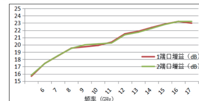
Gain
