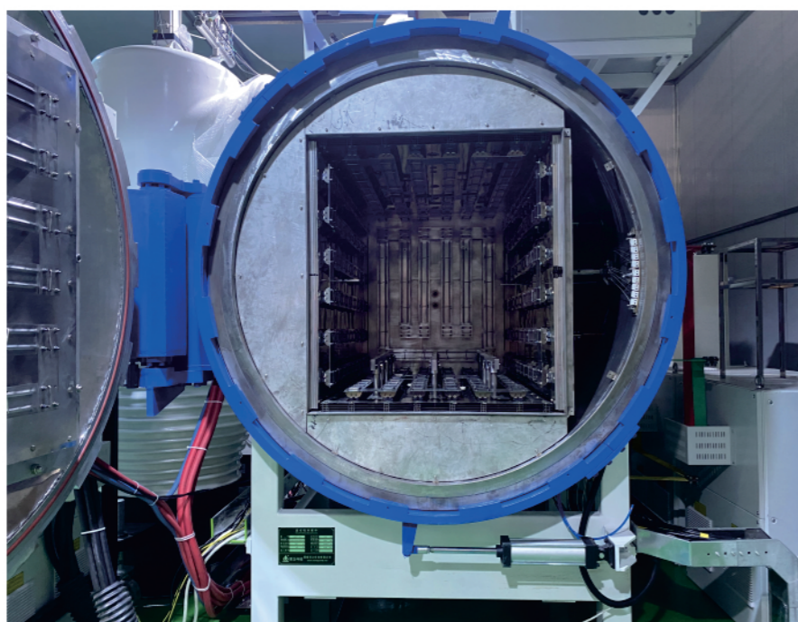
Vacuum Brazing Furnace
