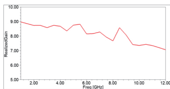
Gain
