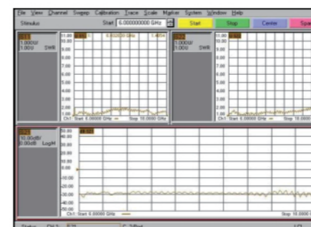
Volt Standing Wave Ratio
