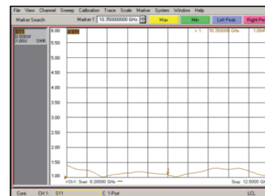
Volt Standing Wave Ratio
