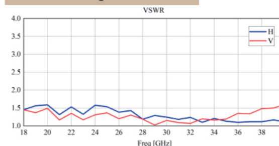
Volt Standing Wave Ratio
