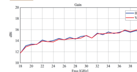
Gain
