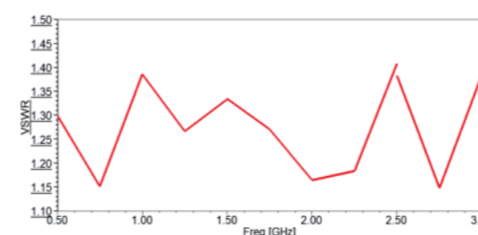
Voltage Standing Wave Ratio
