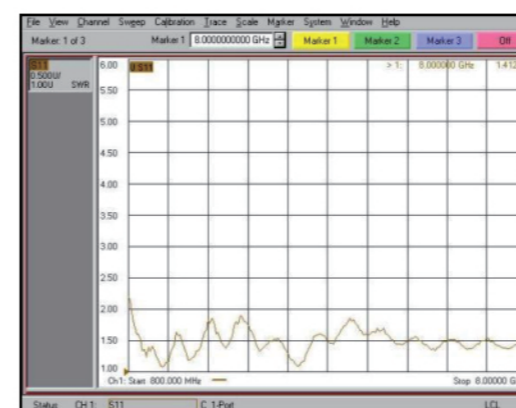
Volt Standing Wave Ratio
